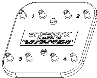
For SAFEMTX Unit with Diffusion Sensor: Calibration Cover Assembly (P/N 10066581)
