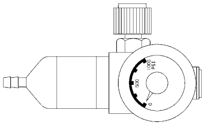
For SAFEMTX Unit with Diffusion Sensor: 0.25 LPM Flow Regulator (P/N 478359)
